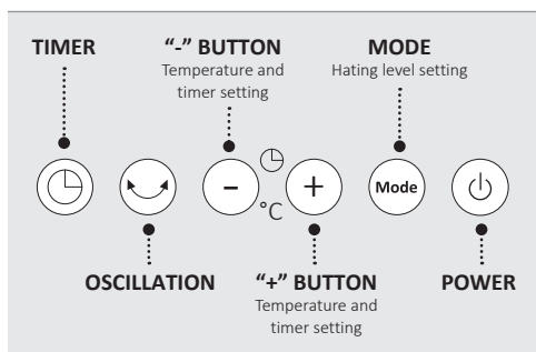
Fig.2: Control unit
