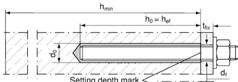
Anchor rod Pre-positioned anchor
