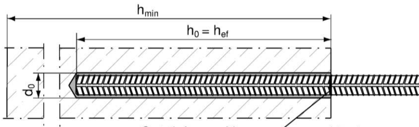
Reinforcing bar
